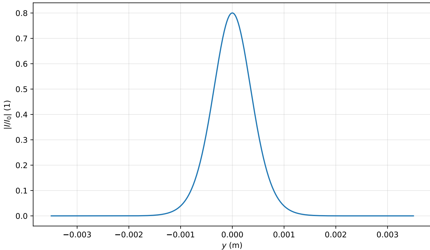
Intensity profile I(x=0, y, z=1.751)/I_0 , P_{in}=0.4P_{cr} , artificial time
